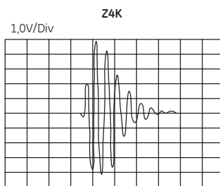
0, 5 \mu S/Div
